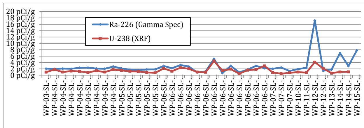
Figure 3-1. Comparison of Ra-226 Gamma Spectroscopy Results to U-238 XRF Results in Vertical Drill Cuttings
