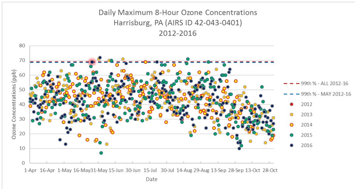
Figure A-14 – Harrisburg, PA Daily Ozone Season Maximums (2012-2016)
